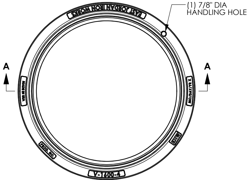
BOTTOM FLANGE VIEW
